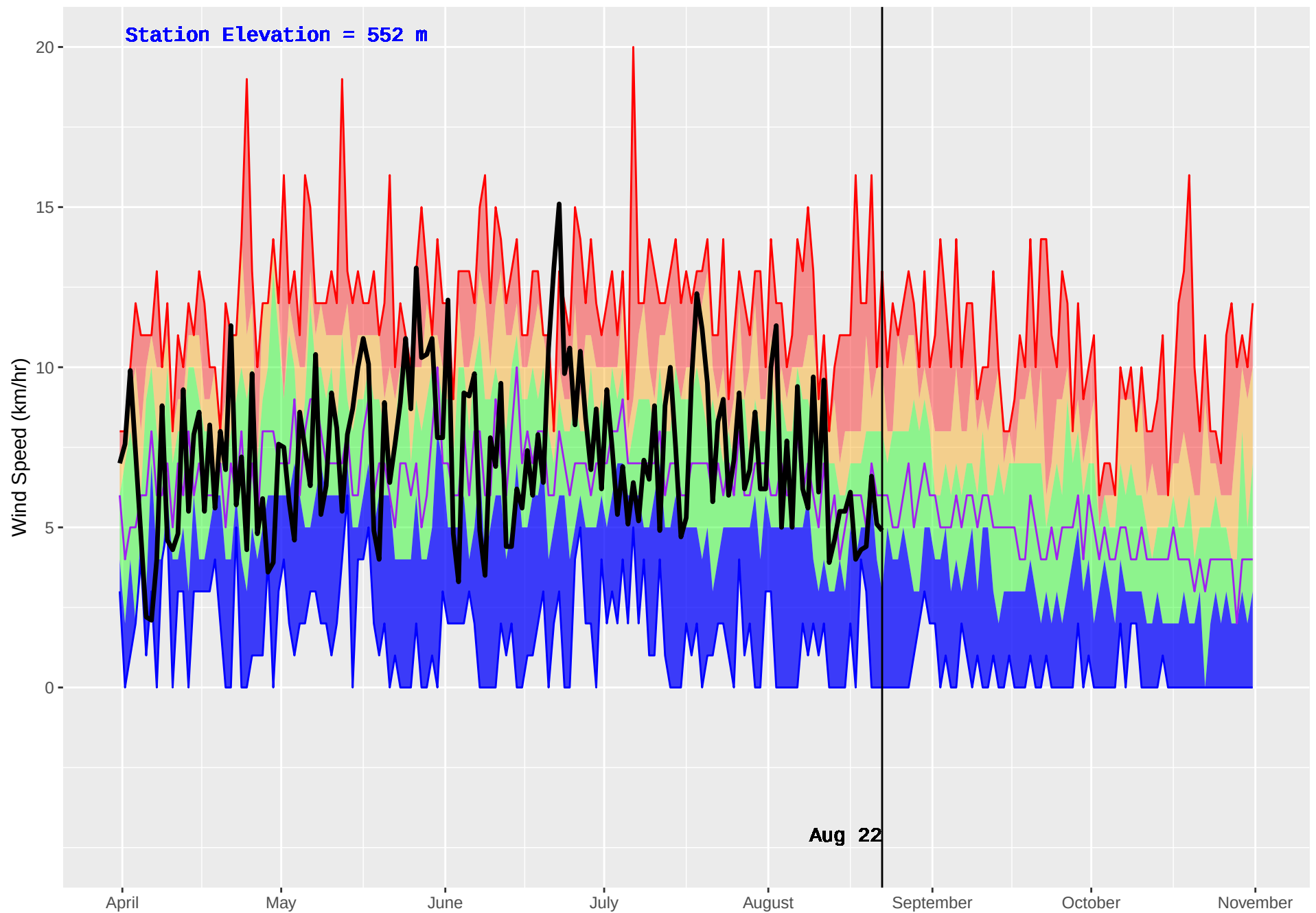
NAHATLATCH (316) : Historical (2001–2016) and Current (2018) Daily Wind Speed
